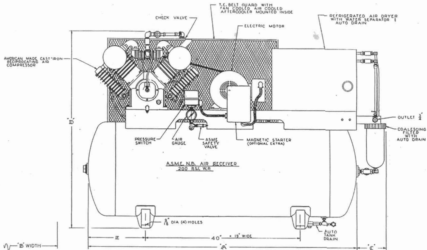
MODEL CD-755-120 AS SHOWN
